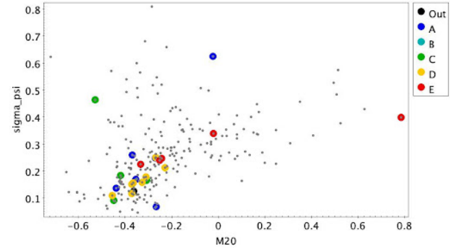
Figure 4: Second moment of light ( M_{20} ) vs spirality ( \sigma_{\text{psi}} ). Larger dots correspond to blue Es, colour coded according to the PPS region they belong to (see diagram from Rhee et al., 2017). Ancient infallers seem to have high spirality, suggesting recent encounters.
