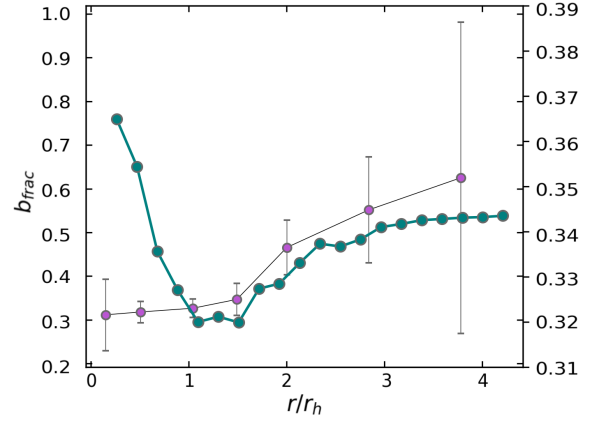
Figure 3: Binary fraction over all stars as a function of radius. The left y-axis corresponds to the magenta curve and measures the binary fraction in concentric rings. The right y-axis corresponds to the green curve and measures the cumulative binary fraction.
