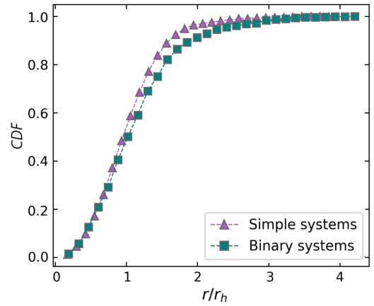
Figure 4: Cumulative radial distribution function of simple and binary population.
